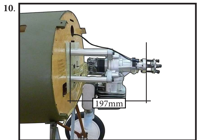
Position the engine with the drive washer (197mm) forward of the firewall.
