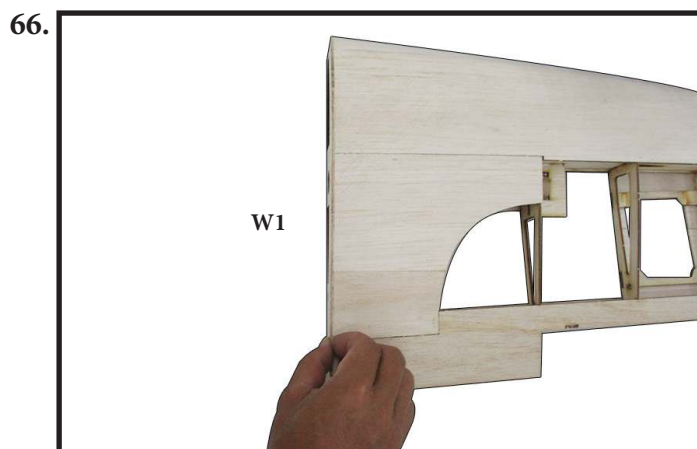
Locate and apply W1 at the root and W10 at the tip. (Photo 66,67).
