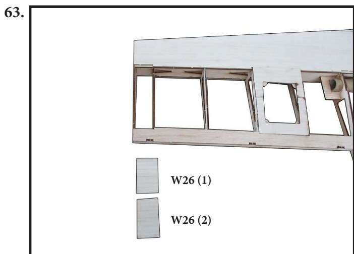
Weld two parts of sheet W26 together to become one. Then, cover to top and bottom side as (photo 63,64).
